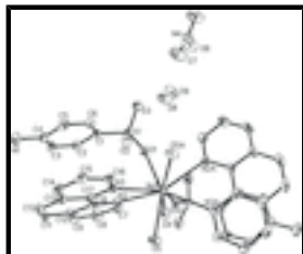
Fig. 1. Molecular structures of the components of (I) showing the atom-labelling scheme and displacement ellipsoids at the 50% probability level. Hydrogen atoms have been omitted for reasons of clarity. Symmetry operation a: 1-x, 1-y, -z.
